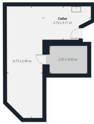
Floor -1
